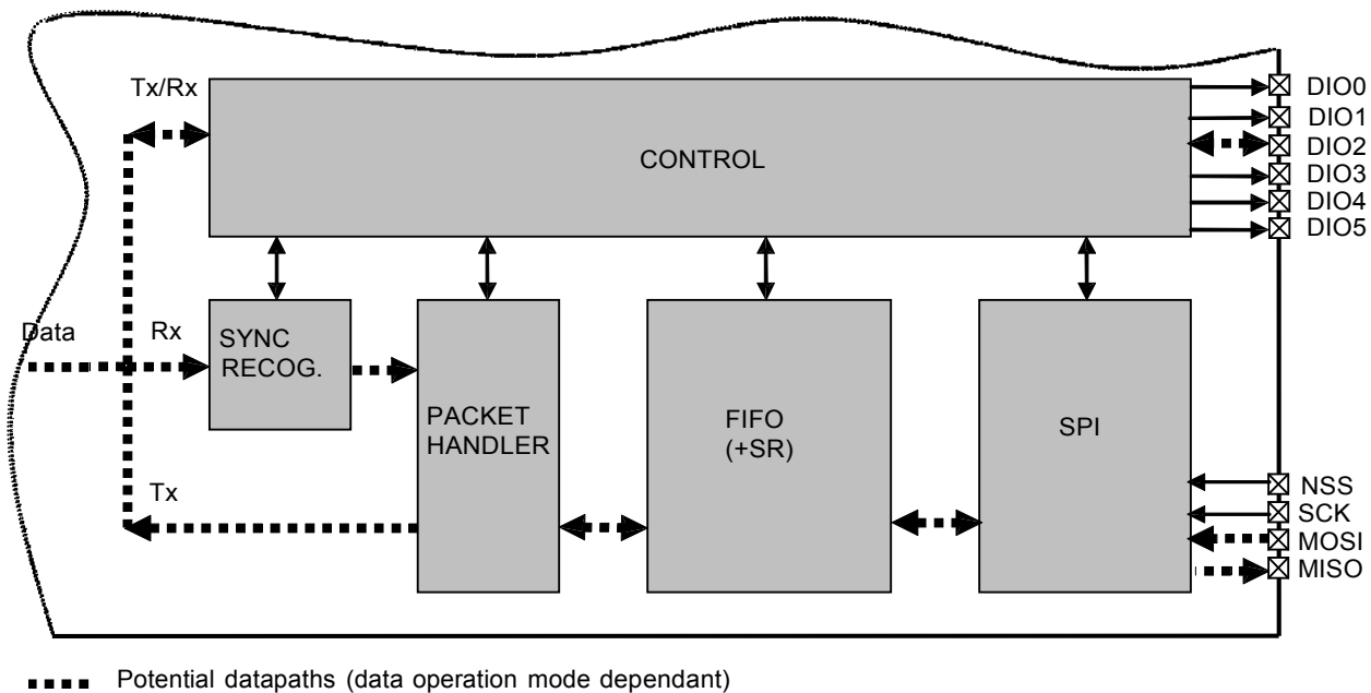
Figure 23. YTX69HC Data Processing Conceptual View
